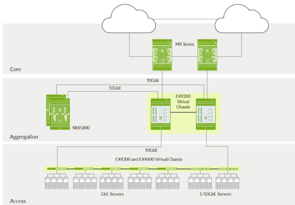
Figure 4: EX4600 provides 10GbE server access in the data center.
