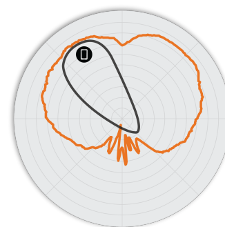
Figure 5. M510 5GHz Elevation Antenna Patterns
